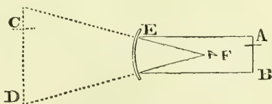
Concave Mirror.
